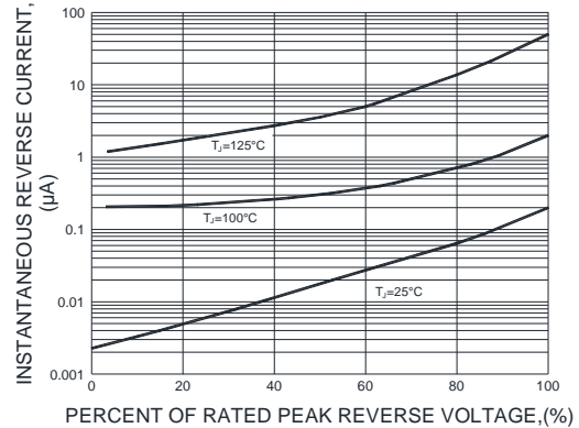
FIG.4-TYPICAL REVERSE CHARACTERISTICS
