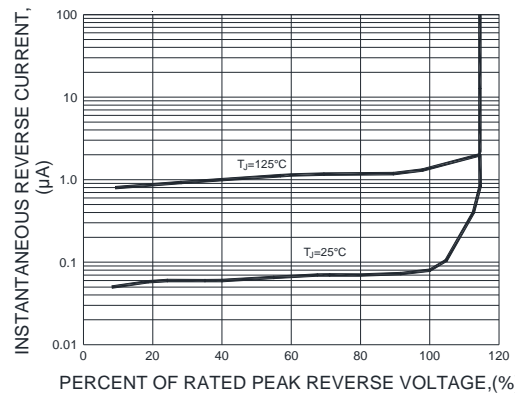
FIG.3-TYPICAL REVERSE CHARACTERISTICS
