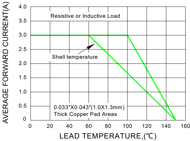
F1G.1-FORWARD CURRENT DERATING CURVE
